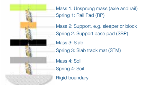
The 4-layer model for Slab Track
