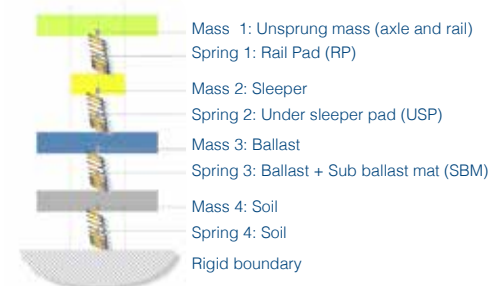
The 4-layer model for Ballasted Track
